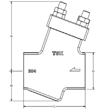
Forged
